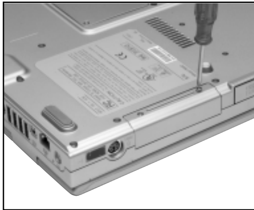
Figure 4.4: Replacing the Hard Disk Drive
