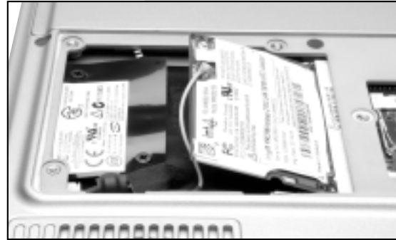
Figure 4.6: Installing the Wireless PCI Card
