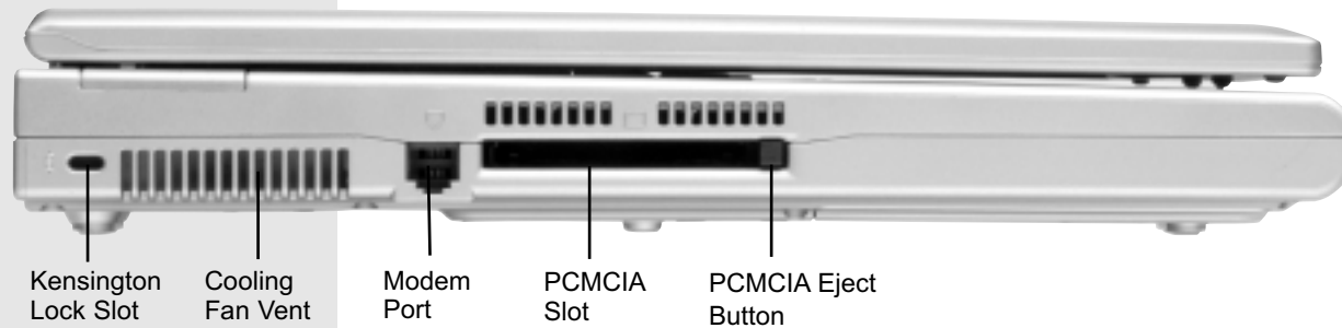
Figure 1.4: Left Side View of the WinBook Notebook
