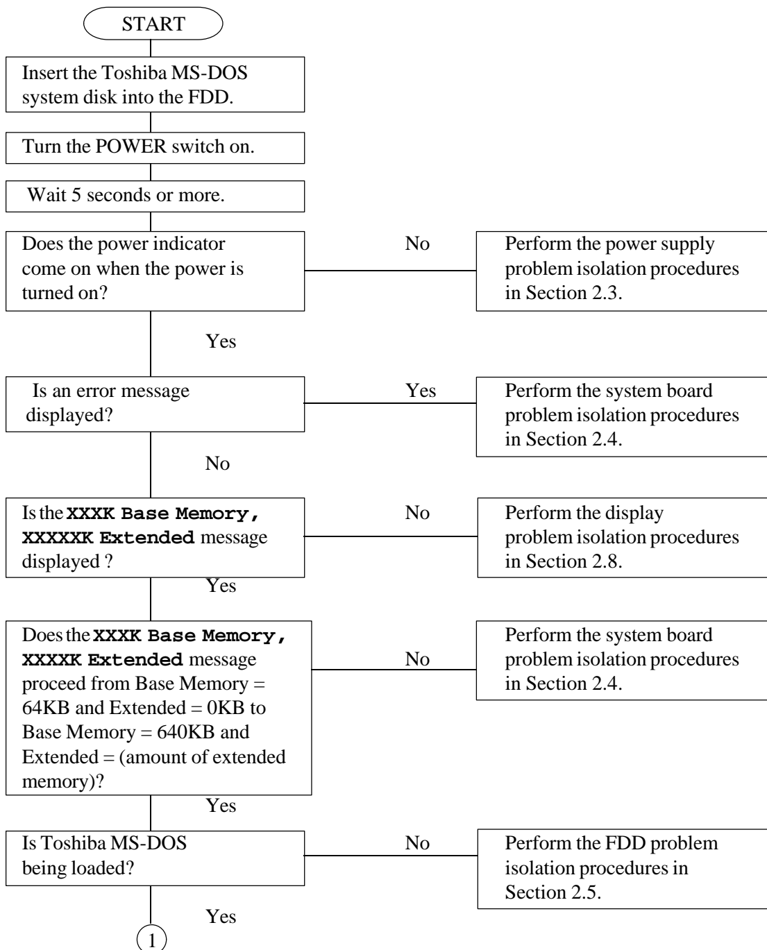
Figure 2-1 Problem isolation flowchart
