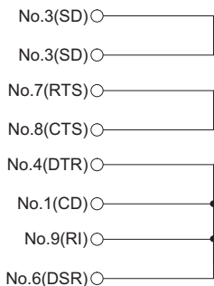
9 pin D-SUB connector
