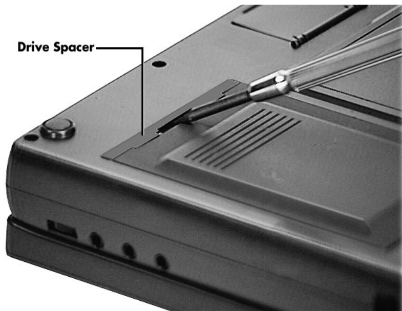
Figure 4-6 Releasing the spacer
