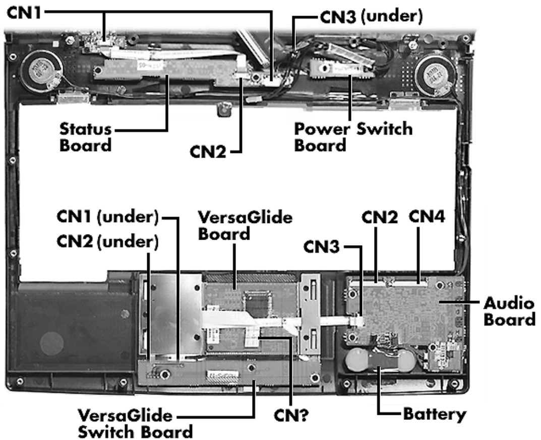
Figure A-2 I/O Board Layout
