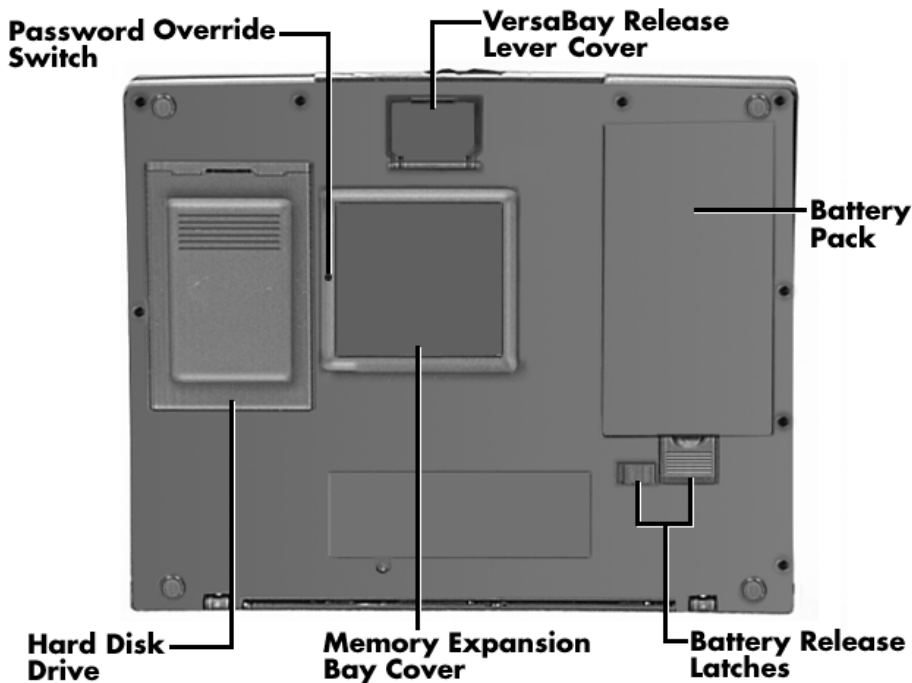
Figure 1-7 Bottom of the system
