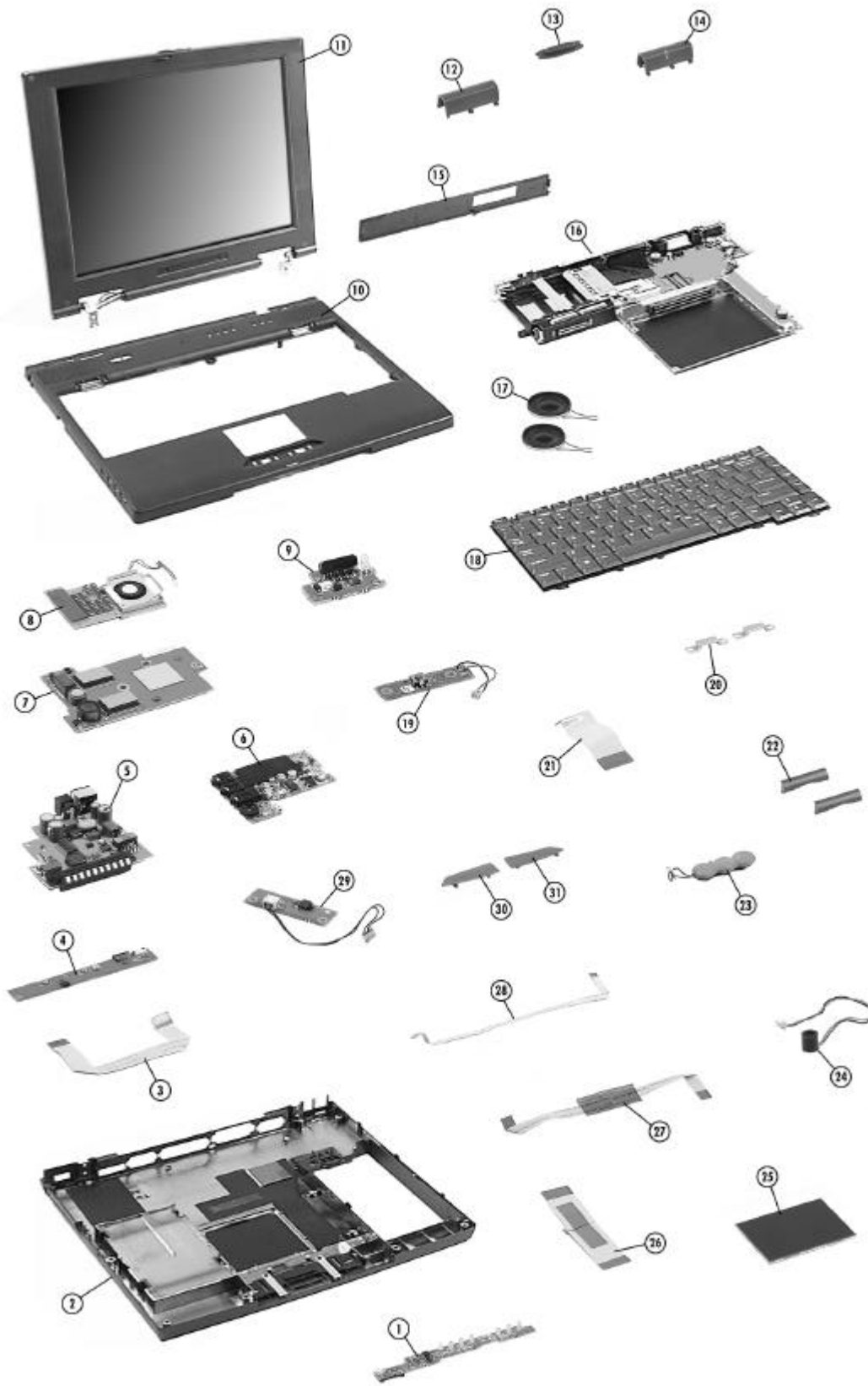
Figure 4-10 NEC Versa 5000 Series Illustrated Parts Breakdown
