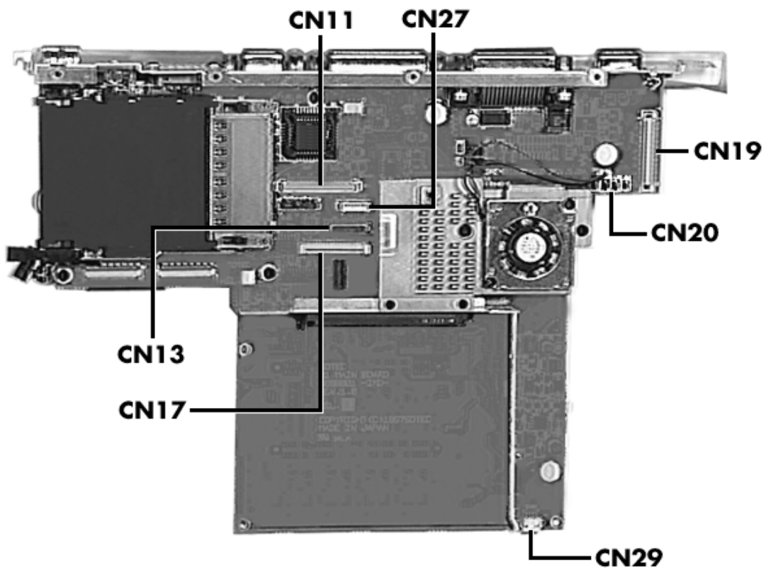
Figure A-1 CPU Board Layout
