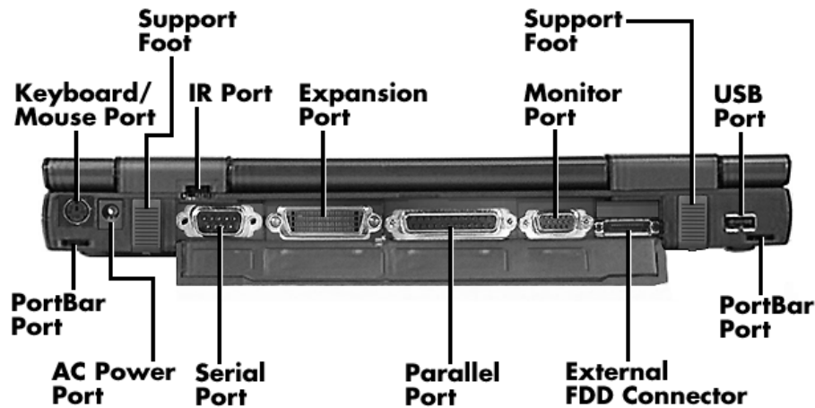
Figure 2-2 Power and I/O Connector Locations
