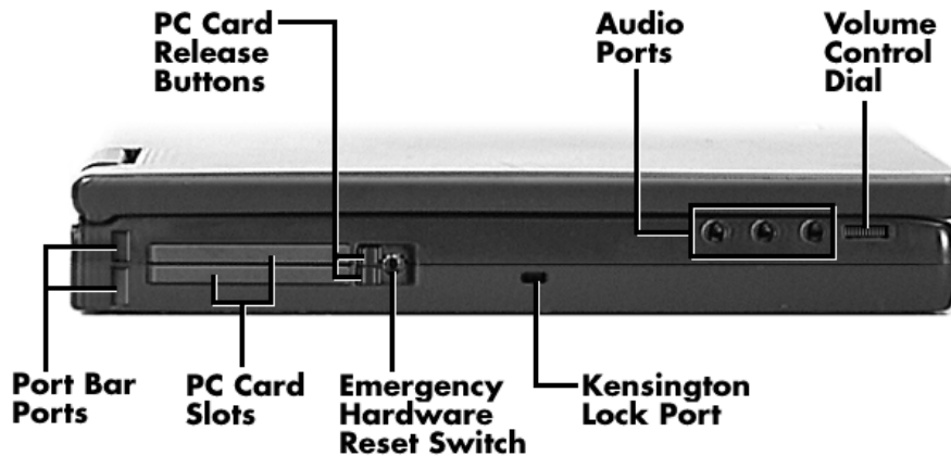
Figure 1-6 Left side features
