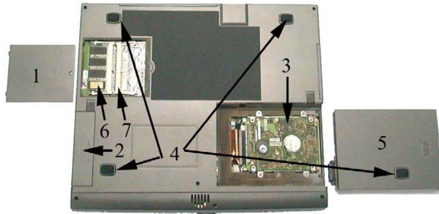
Bottom View of Notebook
