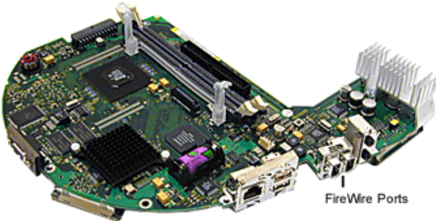
661-2316, 400 MHz, Ver. 2 (revised board, no daughter board)
