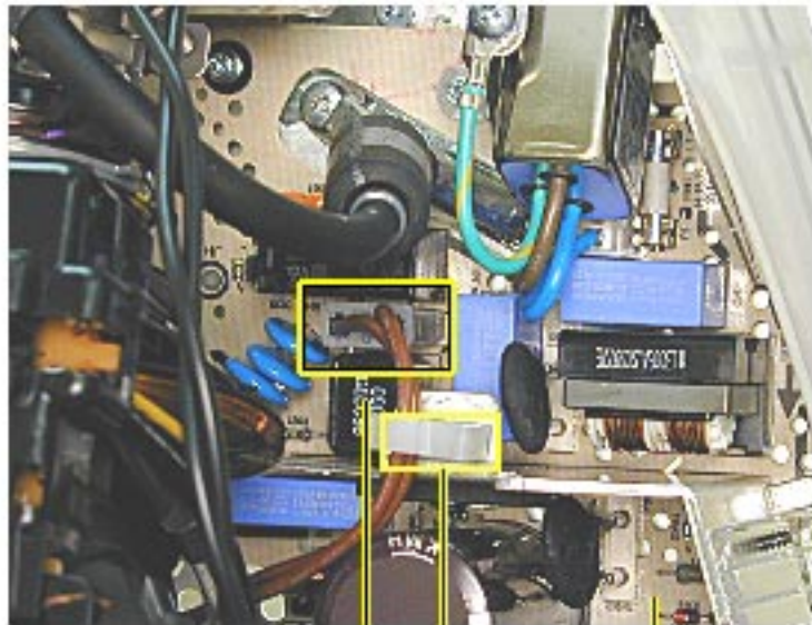
P901 Cable Clamp Power/Analog/Video Board
