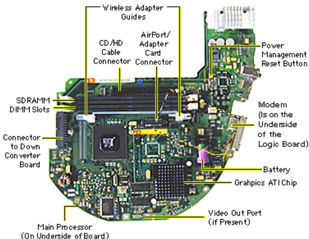
iMac (350 MHz) Logic Board Diagram
