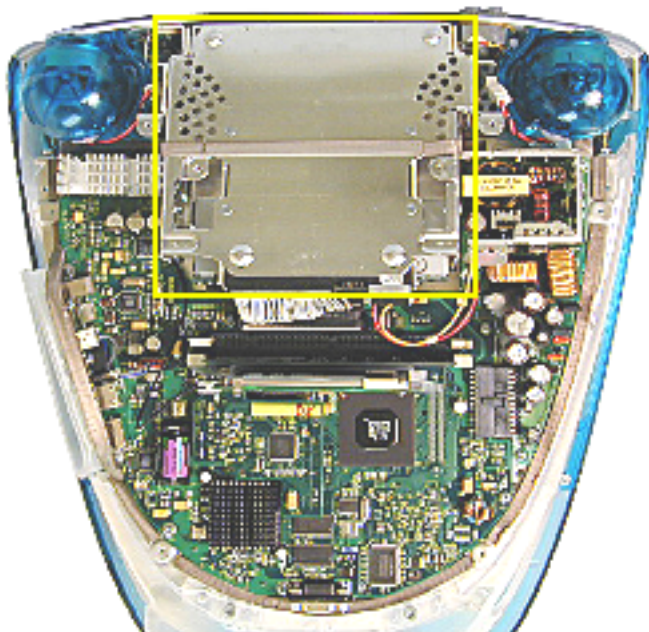
CD/HD Carrier
