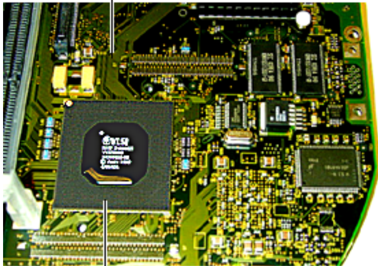
VLSI Chip
