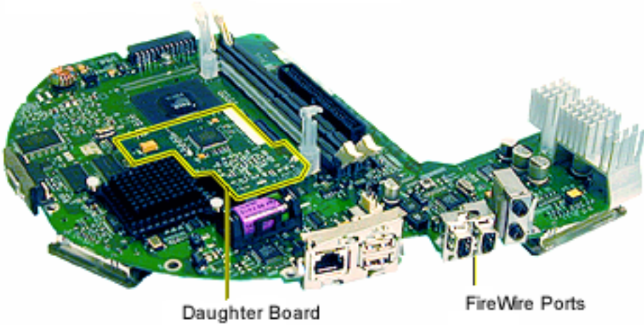
661-2211, 400 MHz, (original board, with daughter board)
